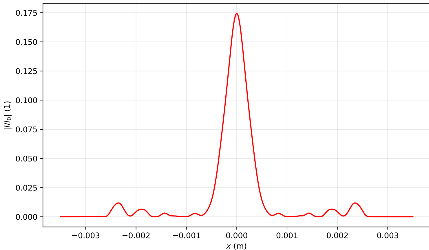
Intensity profile I(x, y = 0, z = 3.025)/I_0 , \text{Pin}=9.0\text{Pcr} , artificial time
